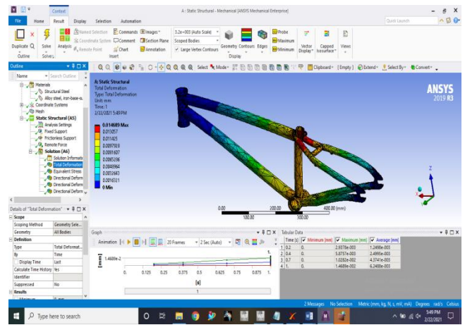
FIG18-TOTAL DEFORMATION
