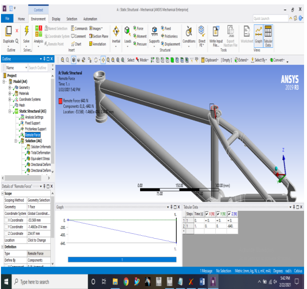
FIG15-REMOTE FORCE
