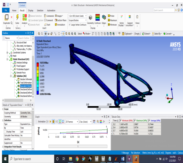
Fig21-Stress
