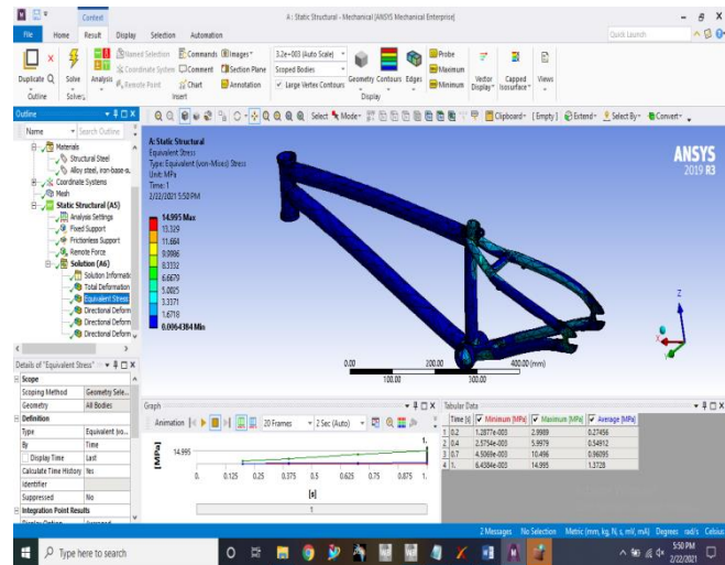
FIG19-STRESS
