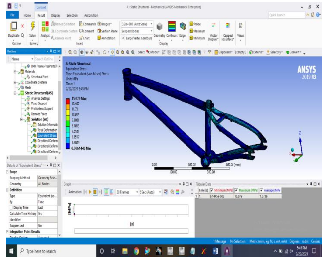
FIG17-STRESS
