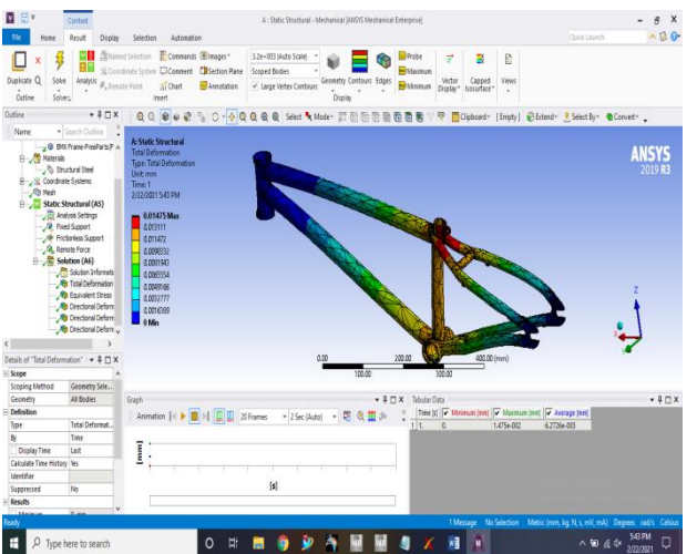
FIG16-TOTAL DEFORMATION
