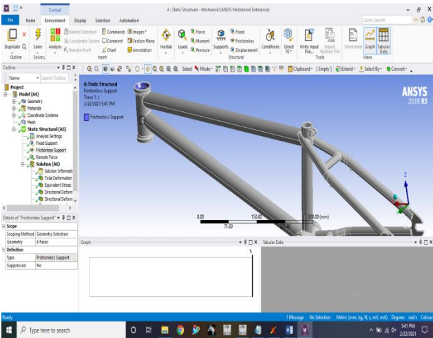
FIG14-FRICTIONLESS SUPPORT
