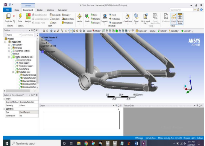
FIG13-FIXED SUPPORT
