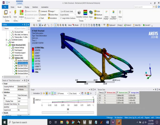
Fig20- Total deformation
